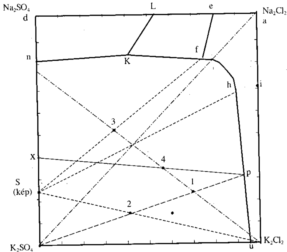
Hình 63: Hệ \text{Na}_2^{2+}, \text{K}_2^{2+} // \text{Cl}_2^{2-}, \text{SO}_4^{2-}, \text{H}_2\text{O}, 25^\circ\text{C} .
