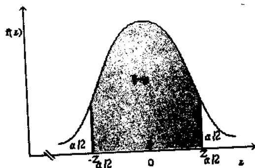
Hình 6.1 P(-z_{\alpha/2} < Z < z_{\alpha/2}) = 1 - \alpha hay P(Z > z_{\alpha/2}) = P(Z < -z_{\alpha/2}) = \alpha/2
