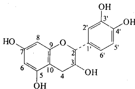
1: ( \pm )-catechin
